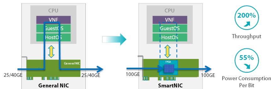
Figure 3-6 Acceleration Solution of SmartNIC
