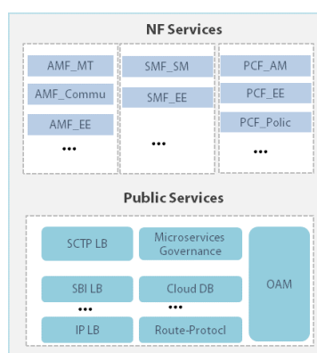
Figure 3-15 Cloud Native &amp; Microservice Architecture
